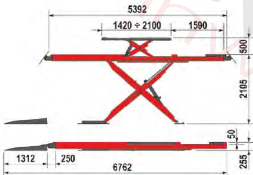
ERCO X5000 CT LT PT
