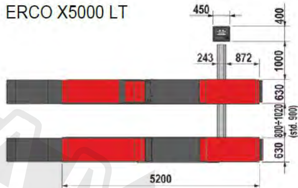
ERCO X5000 CT LT
