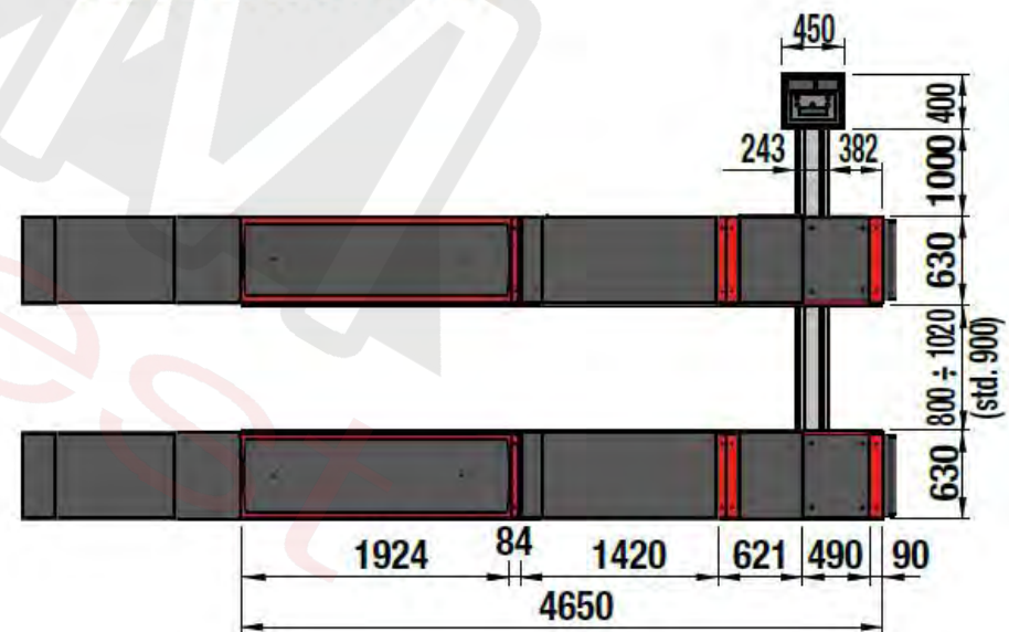
ERCO X4300 CT LT
